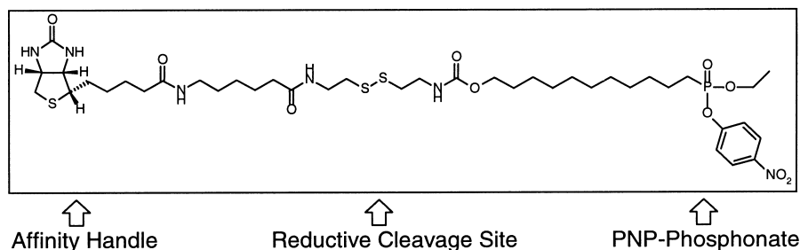
Figure 1. Structure of the affinity label: a 4-nitrophenyl activated phosphonate, that is, a suicide substrate of lipolytic enzymes is connected to a biotin moiety (affinity handle) through a spacer containing a disulfide bridge (reductive cleavage site).
