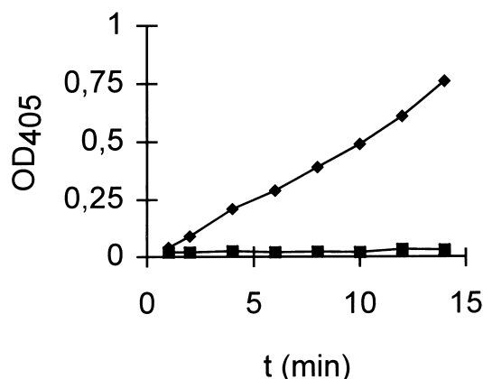
Figure 3. Lipolase ® , inactivated by the inhibitor ( 8 ), and the affinity of inactivated Lipolase ® for streptavidin coated surfaces, has been quantified by ELISA using horseradish peroxidase (HRP) conjugated anti-Lipolase ® antibodies. Protocol: 1. streptavidin, 2. Lipolase ® , 3. \alpha -Lipolase ® , 4. HRP \alpha ( \alpha -Lipolase ® ), 5. detection reagent (1,2-phenylenediamine dihydrochloride). The figure shows the colour development at 405 nm by HRP catalyzed oxidation of 1,2-phenylenediamine dihydrochloride (inhibited Lipolase ® : filled diamonds; active Lipolase ® : filled squares). Thus inhibited Lipolase ® binds to streptavidin coated plates whereas active Lipolase ® does not.
