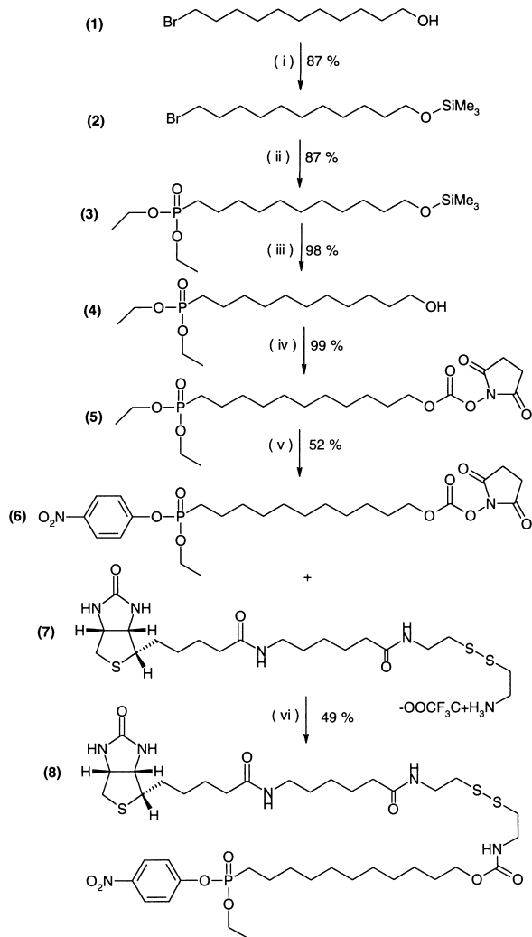
Scheme 1. Reagents and conditions: (i) \text{Me}_3\text{SiCl} , \text{Et}_3\text{N} , \text{CH}_2\text{Cl}_2 /ether; (ii) (\text{EtO})_3\text{P} /reflux; (iii) \text{H}_2\text{SO}_4 /acetone; (iv) 1. \text{COCl}_2 , 2. N -hydroxy-succinimide/ \text{Et}_3\text{N} ; (v) 1. (\text{COCl})_2 , 2. 4-nitrophenol/ \text{Et}_3\text{N} ; (vi) \text{DMF} / \text{Et}_3\text{N} .
