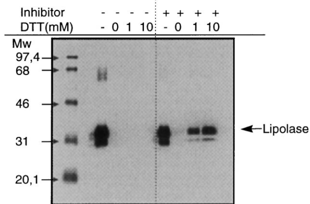
Figure 4. Elution of inhibited or active Lipolase ® from streptavidin coated magnetic beads after washing and incubation with buffer containing DTT (dithiothreitol) at indicated concentrations. M: marker; Lane 1: 25 ng active Lipolase ® ; Lanes 2–4: elution of non-inhibited Lipolase ® after wash and incubation with buffer containing 0, 1, or 10 mM DTT. Lane 5: 25 ng inhibited Lipolase ® ; Lanes 6–8: elution of inhibited Lipolase ® after wash and incubation with buffer containing 0, 1, or 10 mM DTT. Lipolase ® capture and detection was performed as described in experimental procedures.
